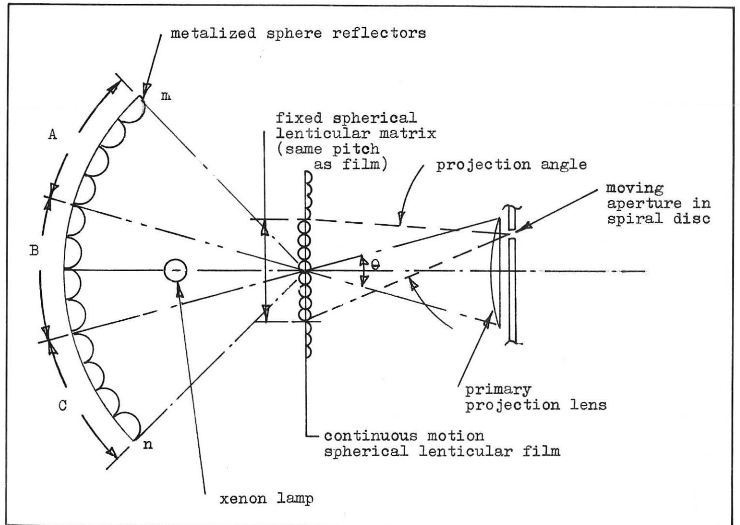
FIGURE 36: Elevation view of projection
