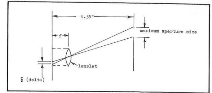
FIGURE 35: Projection lens f-number determination
