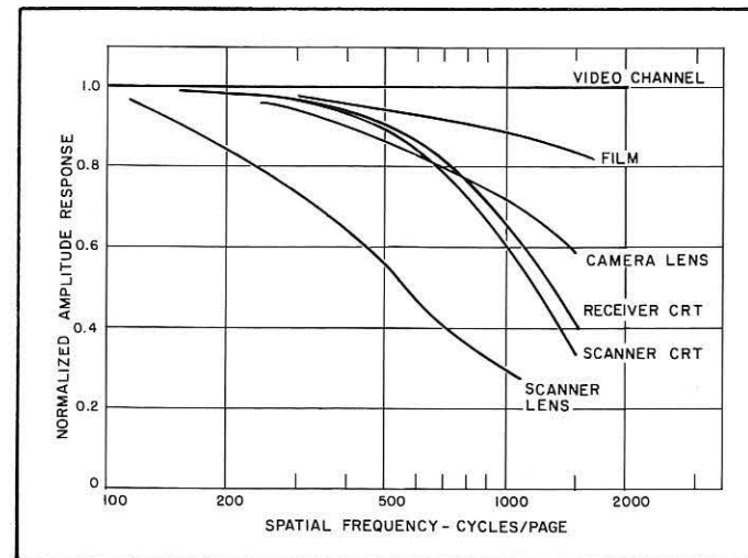
FIGURE 19: Component MTF's in Vertical Scanning Direction.
