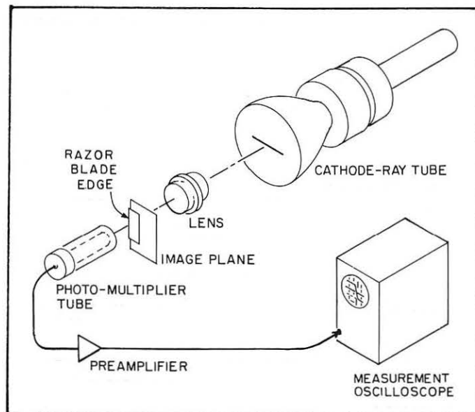
FIGURE 11: Test Setup for Making Edge-Response Measurements
