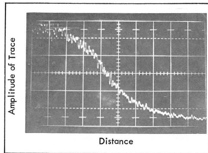
FIGURE 12: Edge-Response Measurement of Scanner CRT-Lens
