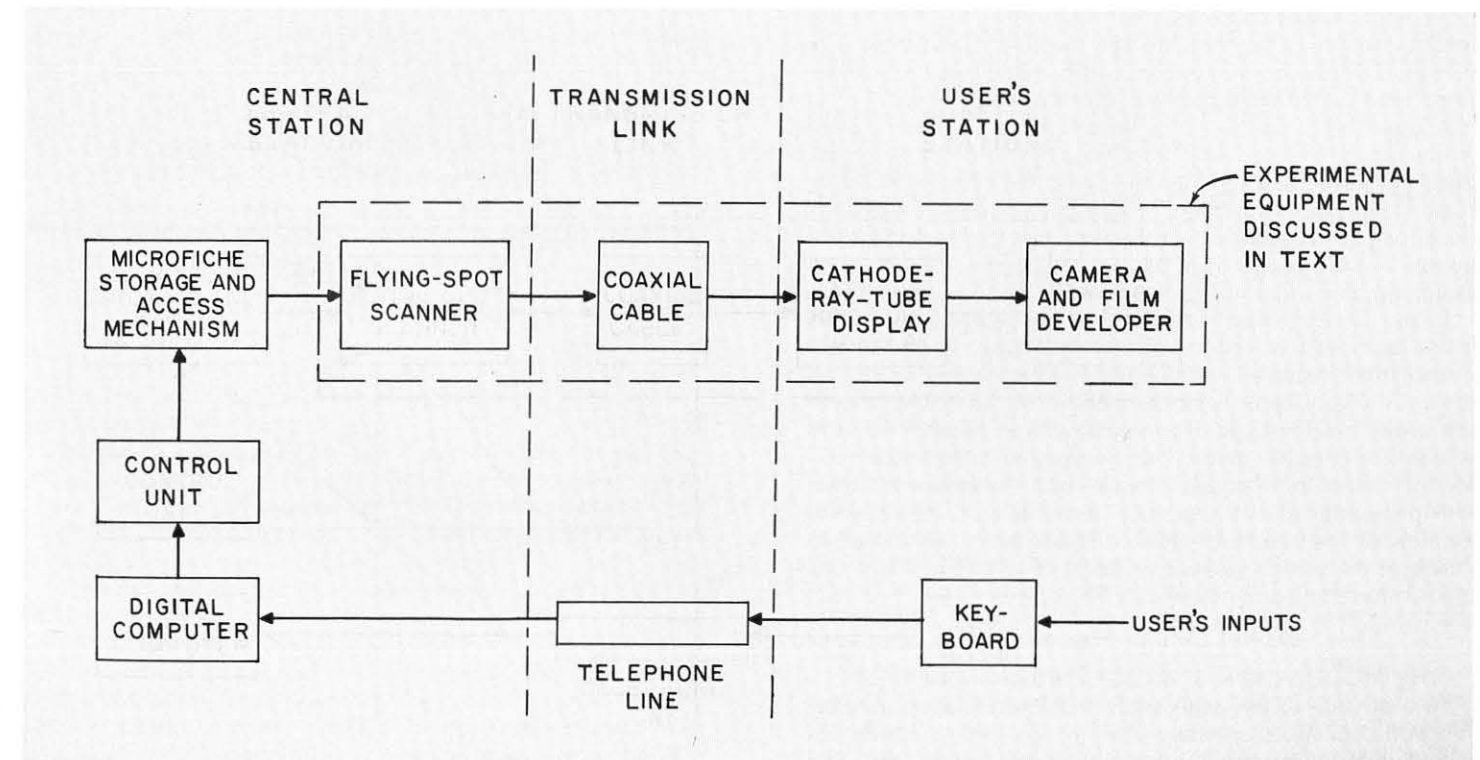
FIGURE 1: Block Diagram of a Remote Text-Access System
