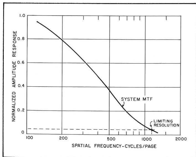
FIGURE 20: System MTF in Vertical Scanning Direction.
