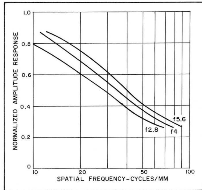
FIGURE 15: Variation of MTF with Lens Aperture.
